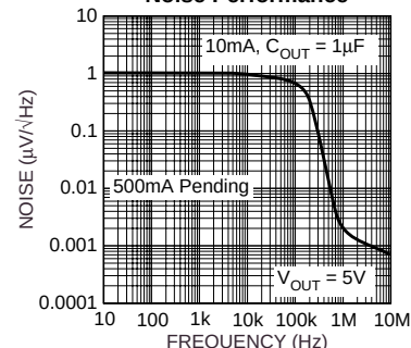
Noise Performance
